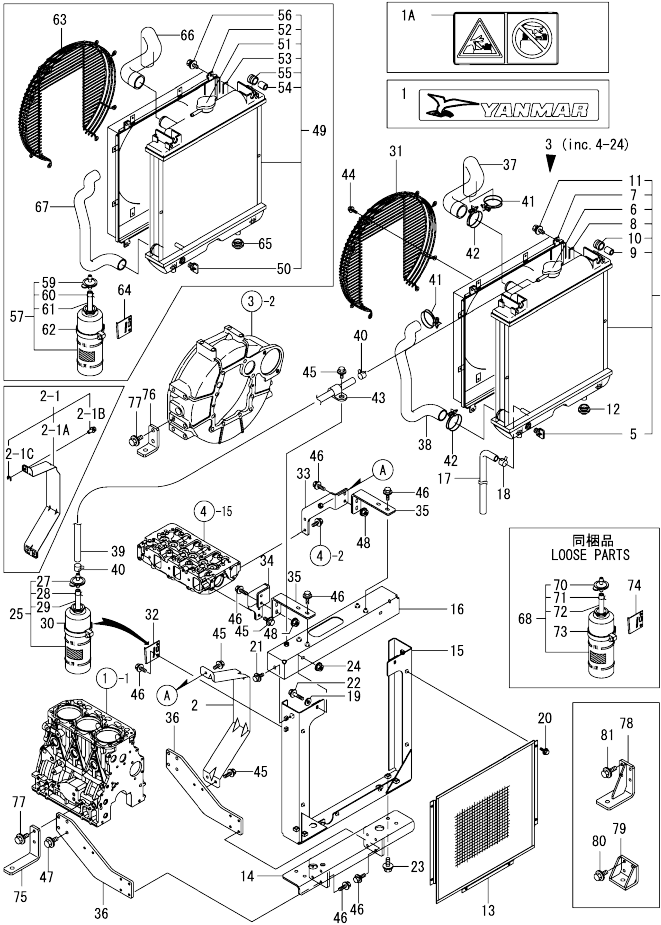
0CW10-M39800 ENGINE Fig.11. RADIATOR
