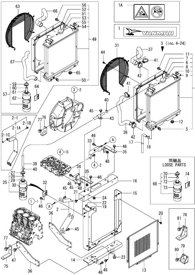
0CW10-M39800 ENGINE Fig.11. RADIATOR
