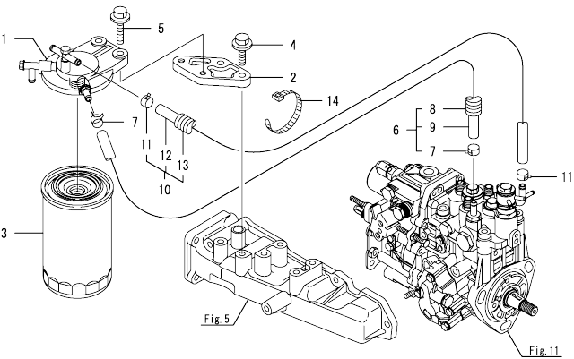
Fig.14. FUEL LINE
