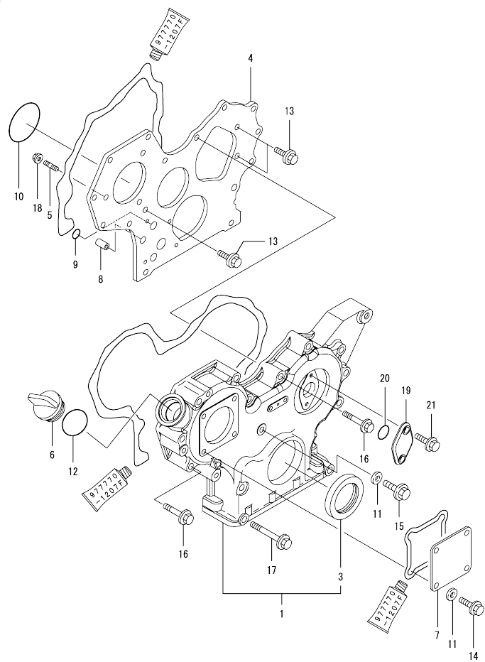
0CW10-M78800 3TNV88-BGECS Fig.2. GEAR HOUSING
