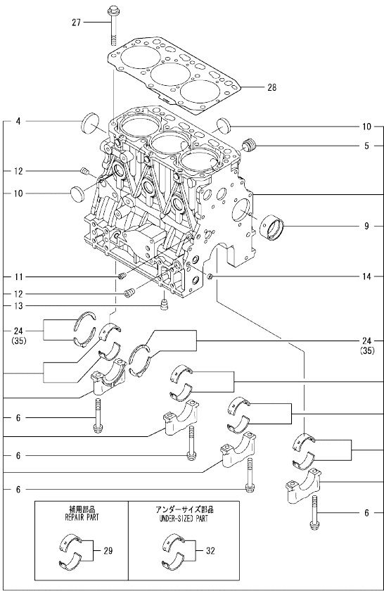
Fig.1. CYLINDER BLOCK
