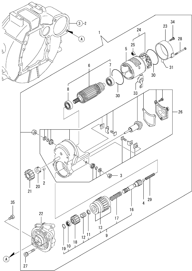
Fig.15. STARTER MOTOR
