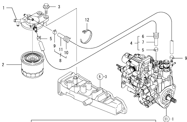
0CW10-M43400 ENGINE Fig.14. FUEL PIPE
