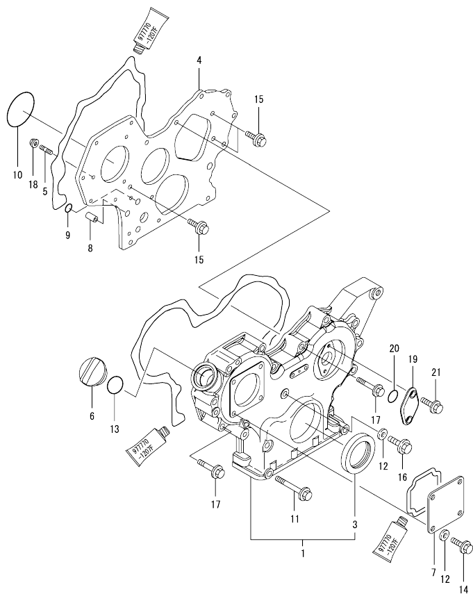
Fig.2. GEAR HOUSING
