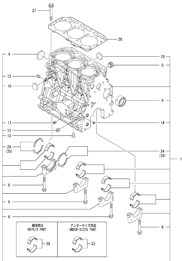
0CW10-M40300 3TNV88-BGGEH Fig.1. CYLINDER BLOCK
