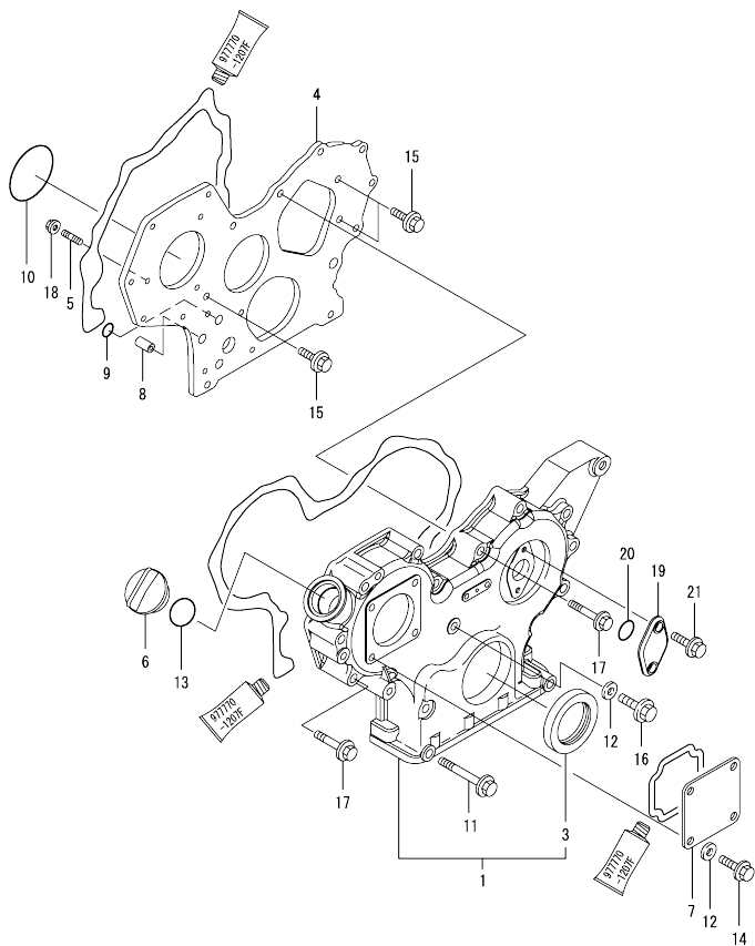
Fig.2. GEAR HOUSING
