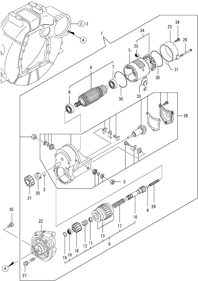
0CW10-M40300 3TNV88-BGGEH Fig.15. STARTING MOTOR
