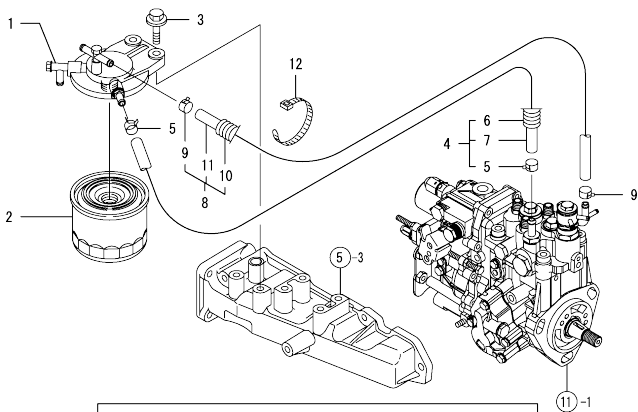
Fig.14. FUEL LINE
