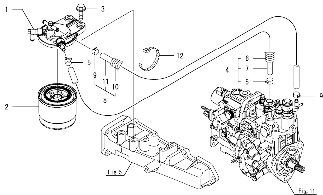
Fig.14. FUEL PIPE
