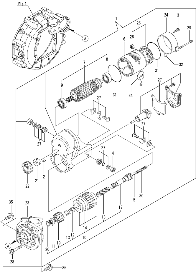
Fig.15. STARTER MOTOR
