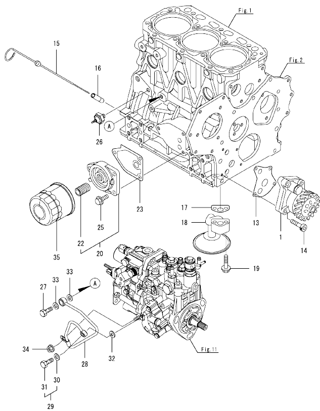
OCD50-M01220 3TNV88-BGGQ Fig.9. LUB. OIL SYSTEM
