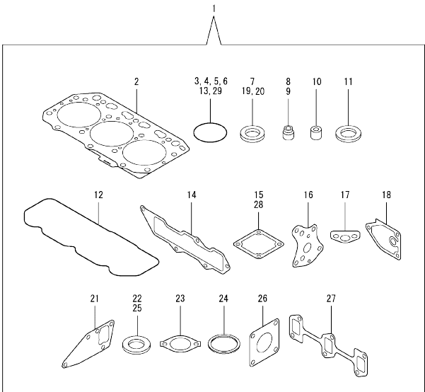
Fig.17. GASKET SET
