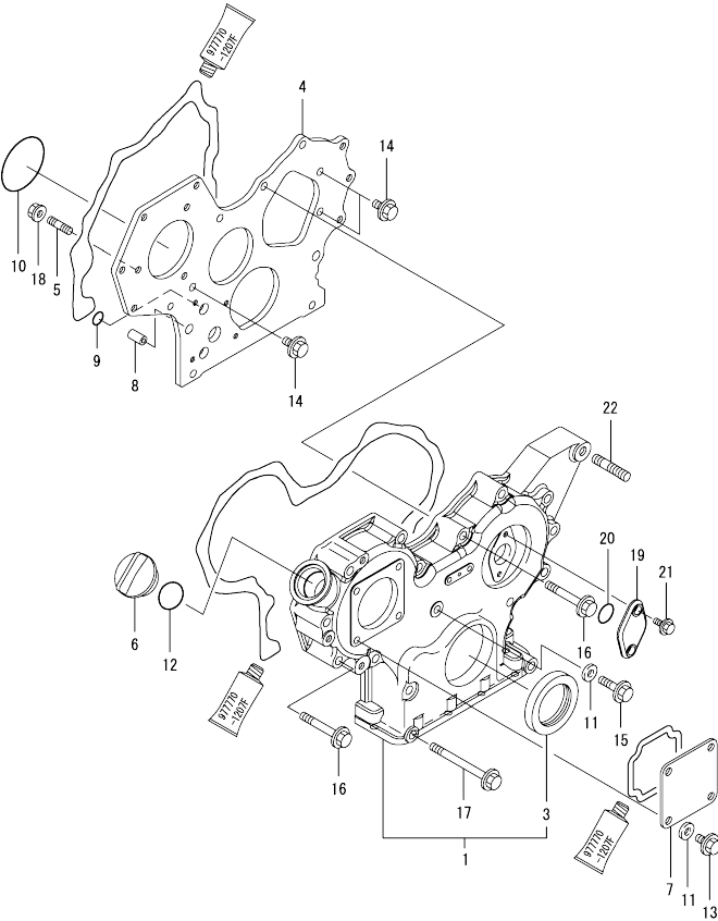
Fig.2. GEAR HOUSING
