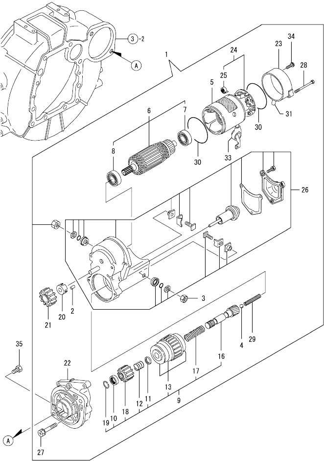
Fig.15. STARTING MOTOR
