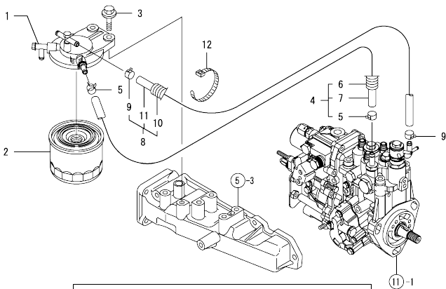
Fig.14. FUEL LINE
