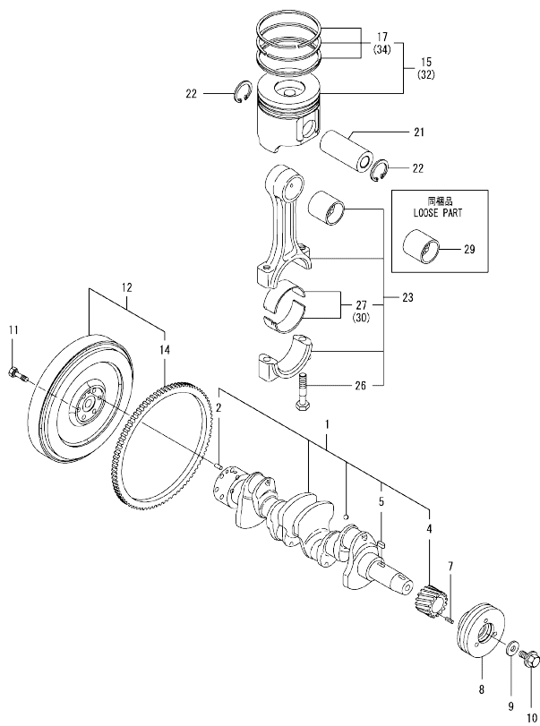
Fig.25. CRANKSHAFT & PISTON
