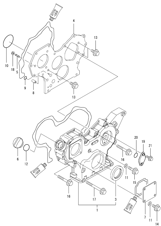
Fig.19. GEAR HOUSING
