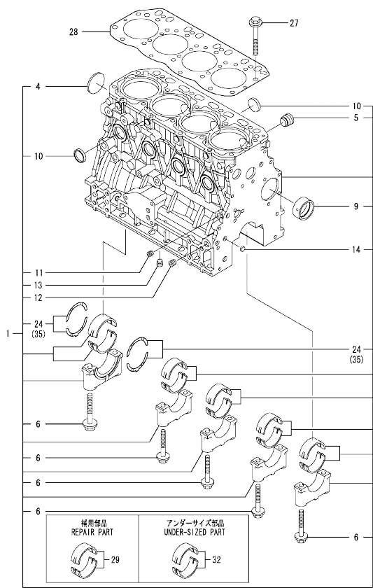
Fig.18. CYLINDER BLOCK
