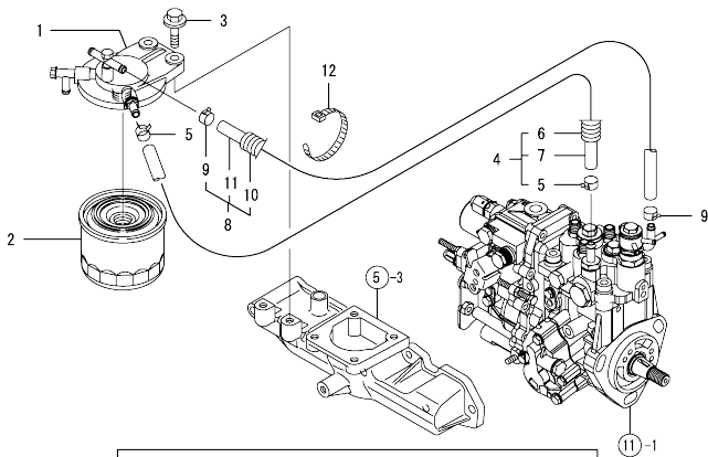
Fig.14. FUEL LINE
