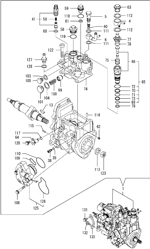
Fig.28. FUEL INJECTION PUMP
