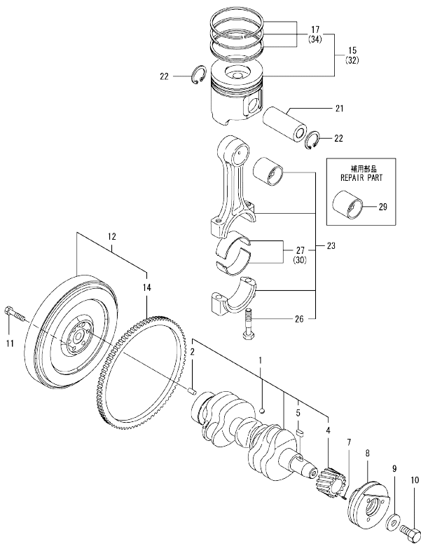
Fig.8. CRANKSHAFT & PISTON
