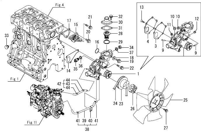
Fig.10. COOLING WATER SYSTEM
