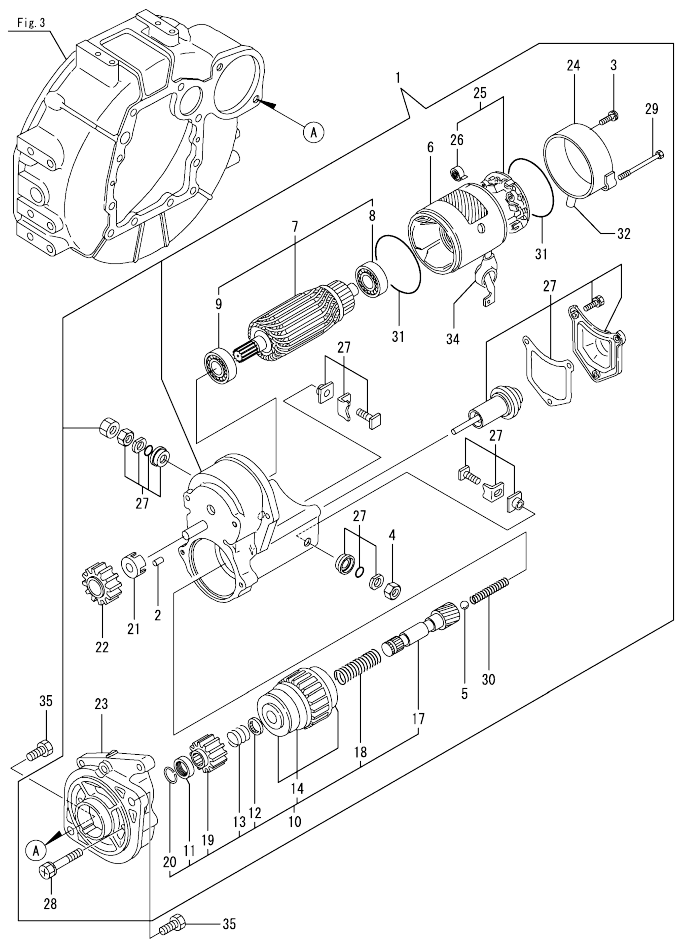
Fig.15. STARTING MOTOR
