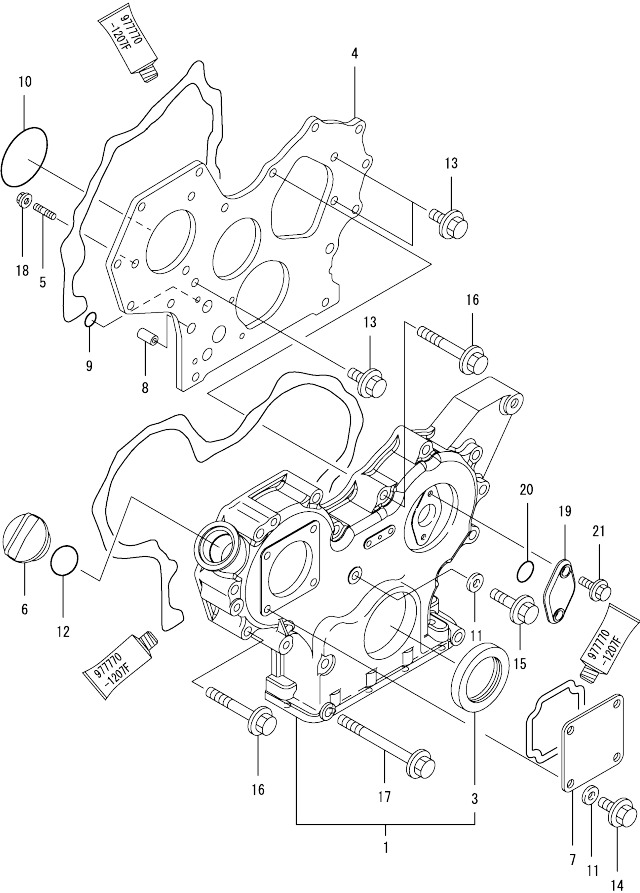
Fig.2. GEAR HOUSING
