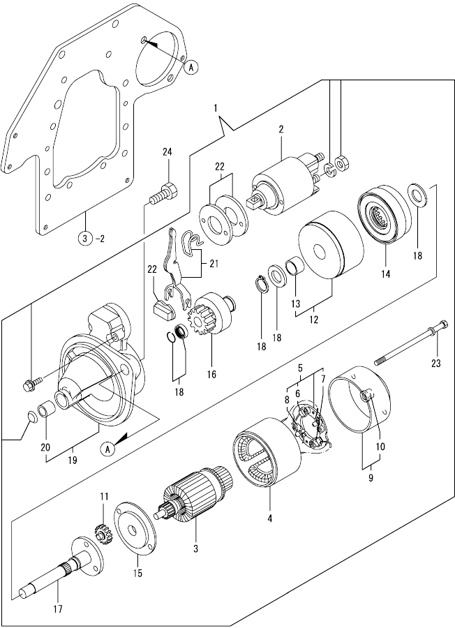
Fig.15. STARTING MOTOR
