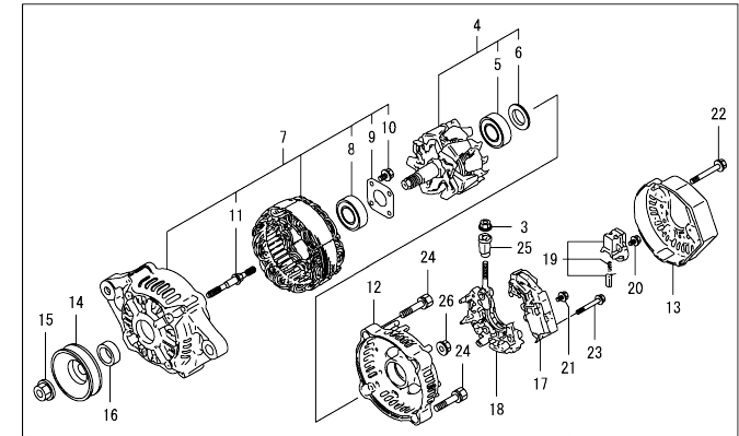
OCD50-M05430 ENGINE Fig.16. GENERATOR
