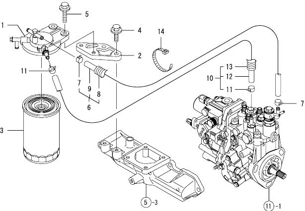
Fig.14. FUEL LINE
