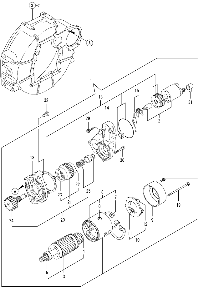
Fig.15. STARTING MOTOR
