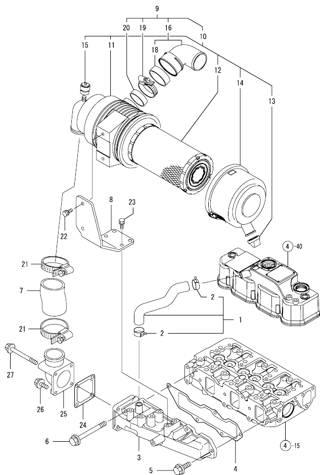
Fig.5. SUCTION MANIFOLD & AIR CLEANER
