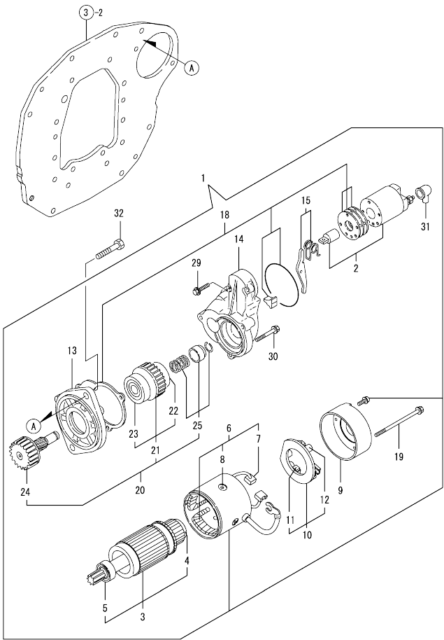
Fig.15. STARTING MOTOR
