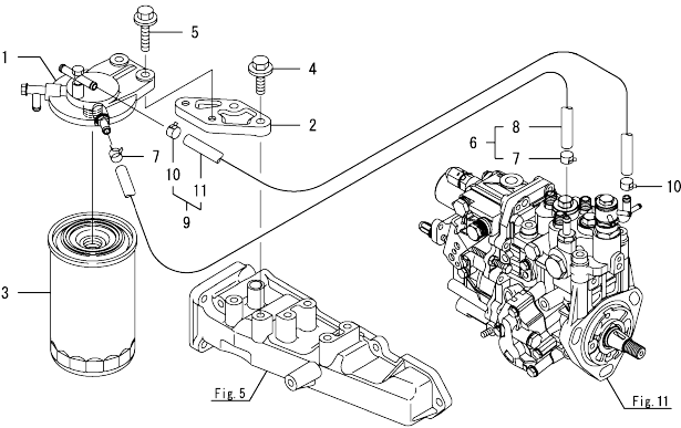
Fig.14. FUEL PIPE
