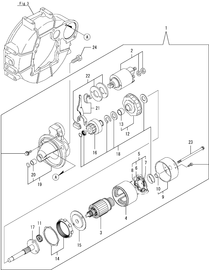
Fig.15. STARTER MOTOR
