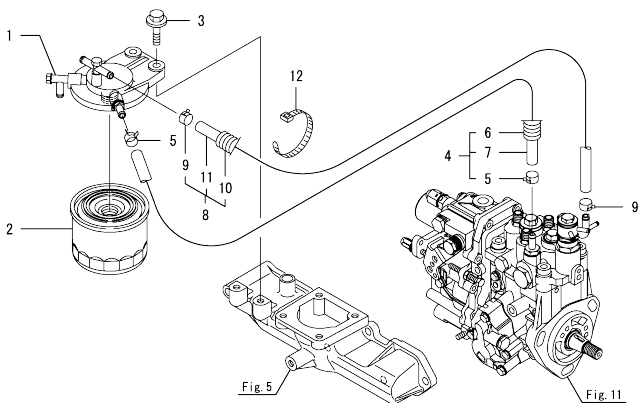
Fig.14. FUEL PIPE
