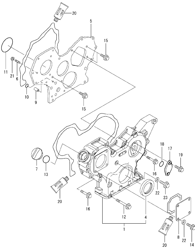
OCD10-M92100 3TNV88-BQIKA Fig.2. GEAR HOUSING
