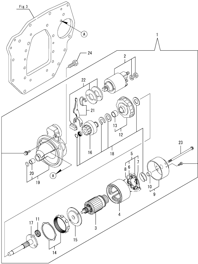
OCD11-M14800 3TNV88-BDHK Fig.15. STARTING MOTOR
