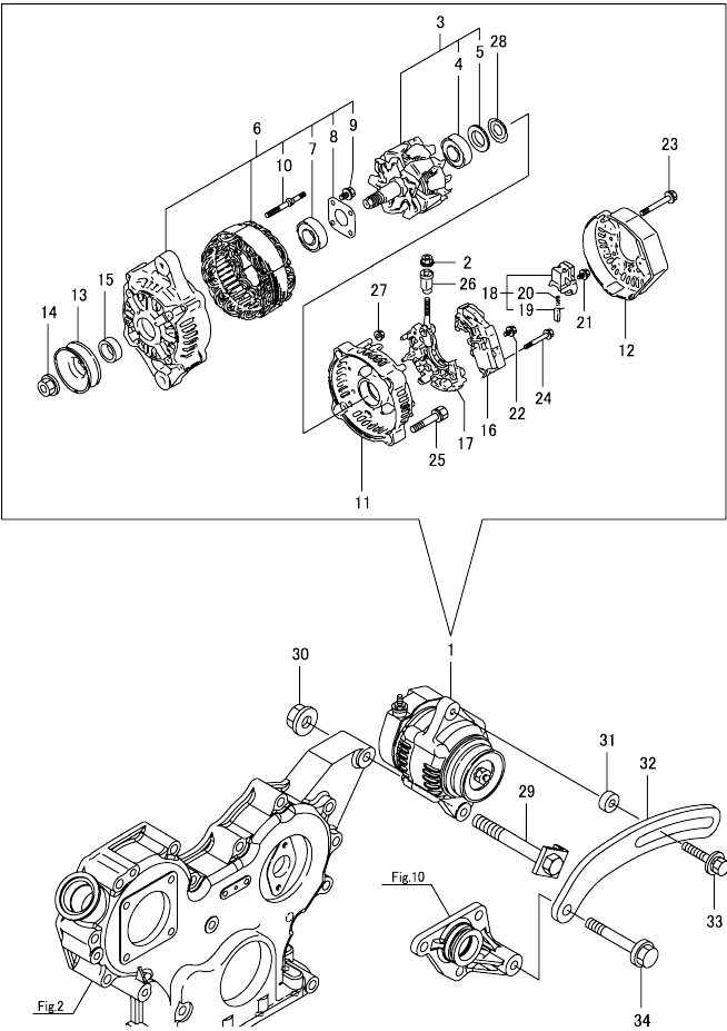
OCD50-M03920 ENGINE Fig.16. GENERATOR
