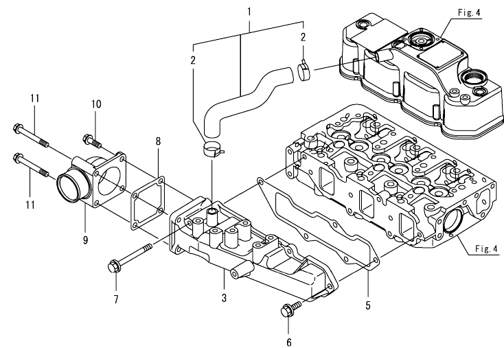
OCD50-M03920 ENGINE Fig.5. SUCTION MANIFOLD
