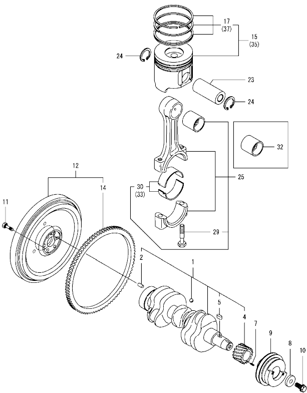
Fig.8. CRANKSHAFT & PISTON
