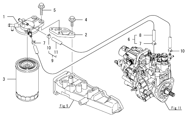
Fig.14. FUEL PIPE
