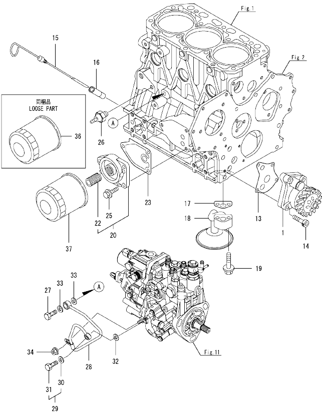
Fig.9. LUB. OIL SYSTEM
