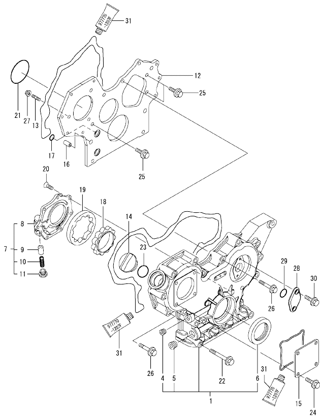
Fig.2. GEAR HOUSING
