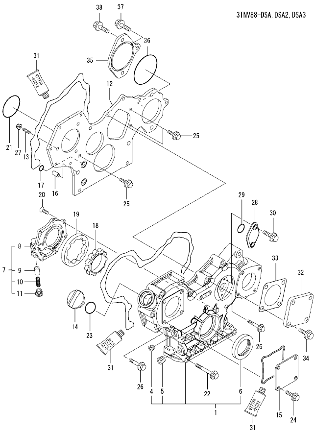
Fig.2. GEAR HOUSING
