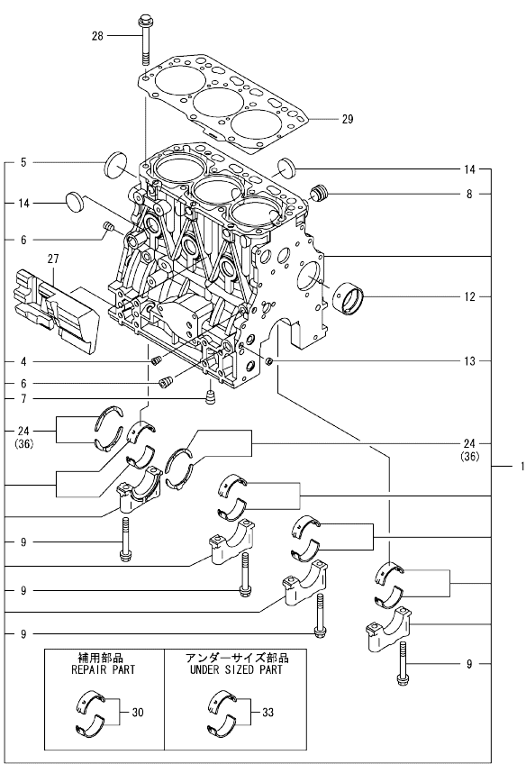
Fig.1. CYLINDER BLOCK
