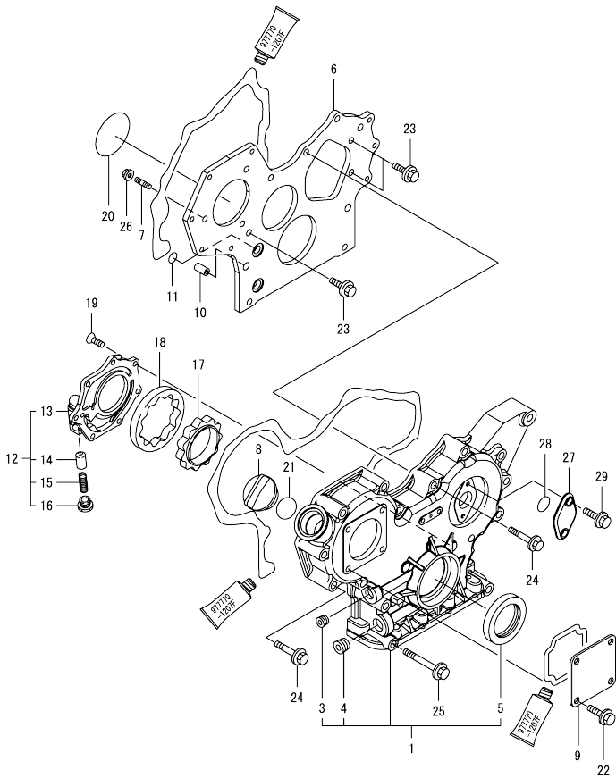
0CW10-M52400 3TNV88-GAGR Fig.2. GEAR HOUSING
