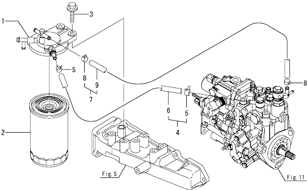
Fig.14. FUEL LINE
