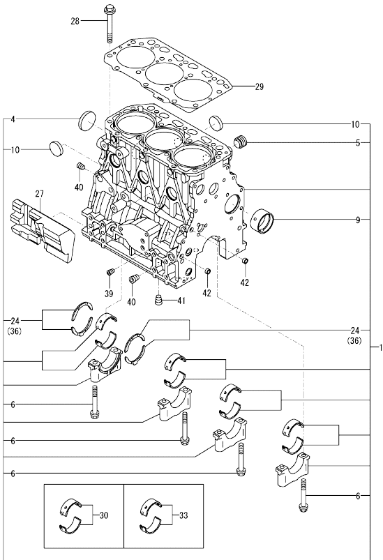
Fig.1. CYLINDER BLOCK
