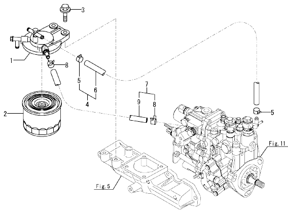
OCD11-M04401 ENGINE Fig.14. FUEL PIPE
