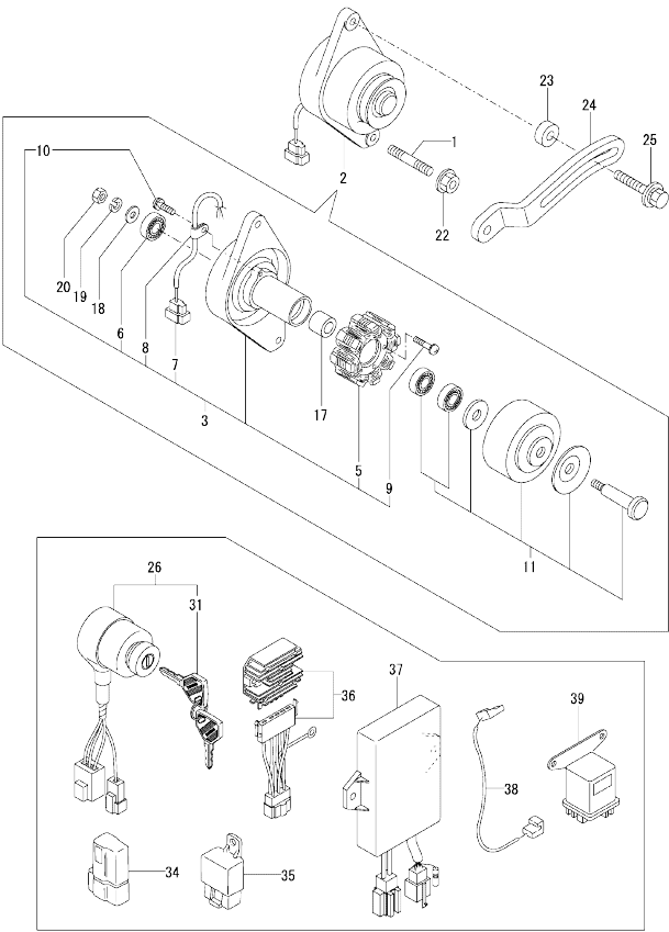
OCD11-M04401 ENGINE Fig.16. GENERATOR
