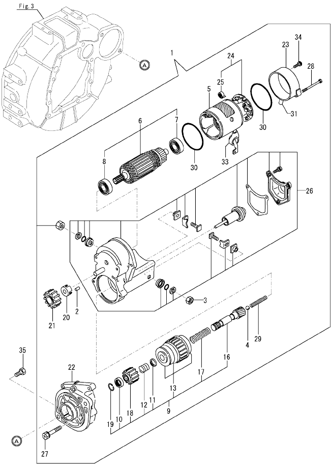
Fig.15. STARTER MOTOR
