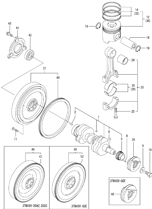
OCR10-M56400 ENGINE Fig.9. CRANKSHAFT & PISTON
