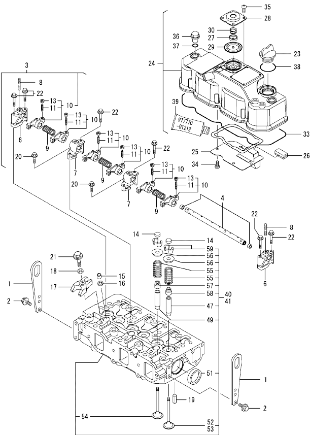
Fig.5. CYLINDER HEAD & BONNET
