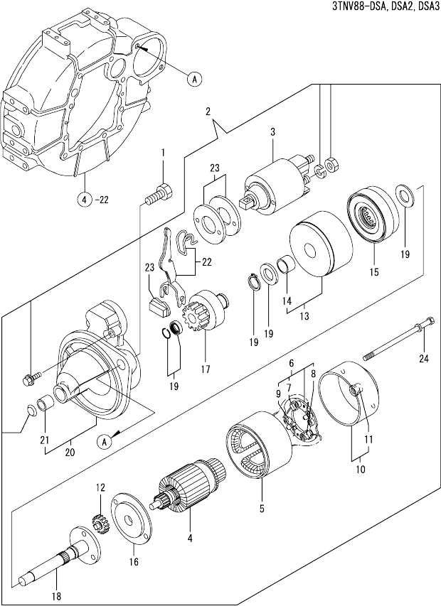
Fig.15. STARTER MOTOR
