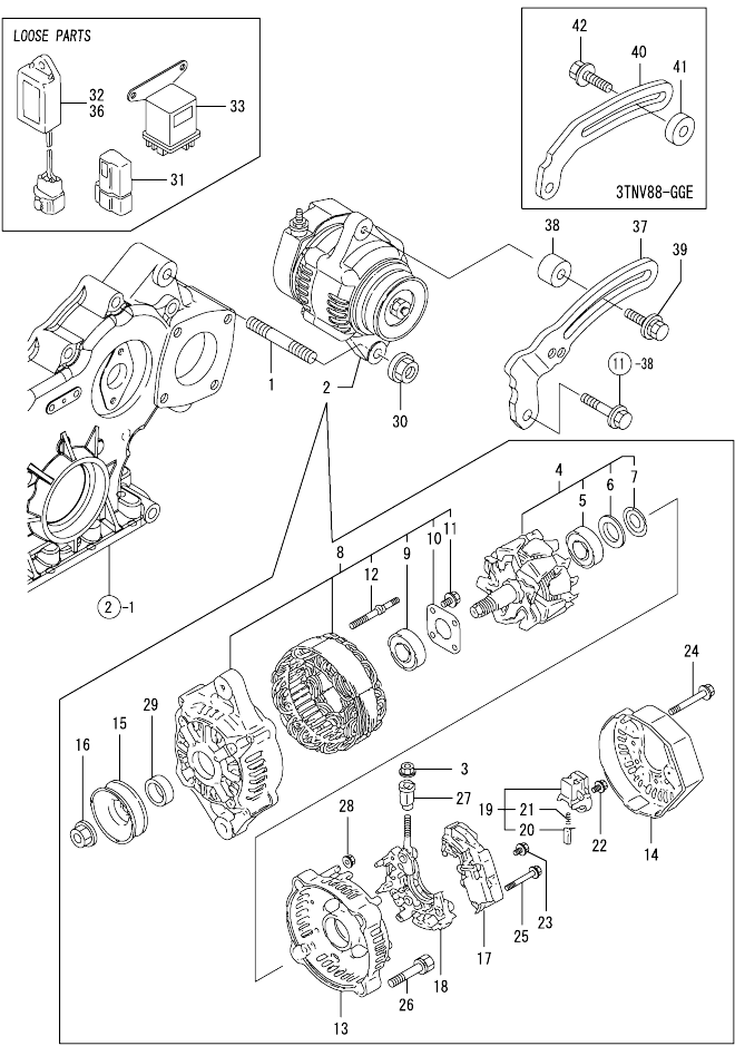
OCR10-M56400 ENGINE Fig.17. GENERATOR
