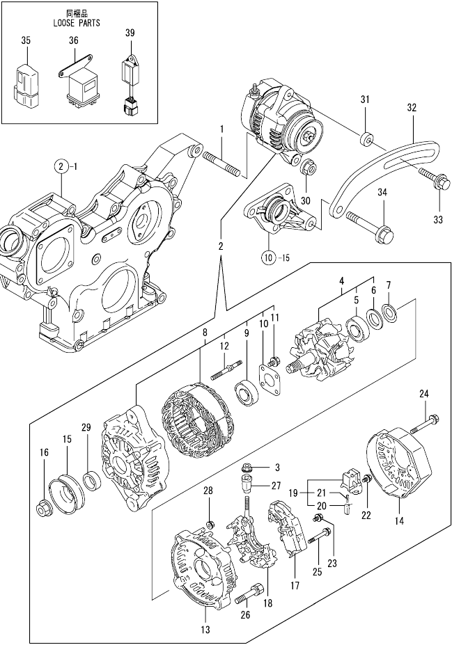
0CW10-M36600 3TNV88-GGEA Fig.16. GENERATOR
