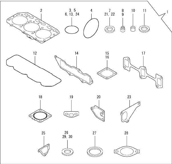
Fig.17. GASKET SET
