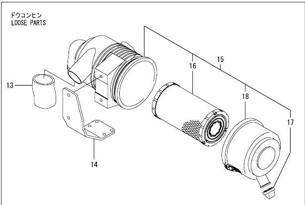
Fig.5. SUCTION MANIFOLD & AIR CLEANER
