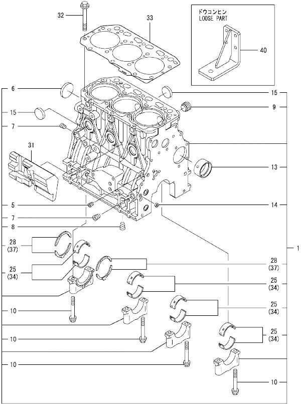
Fig.1. CYLINDER BLOCK
