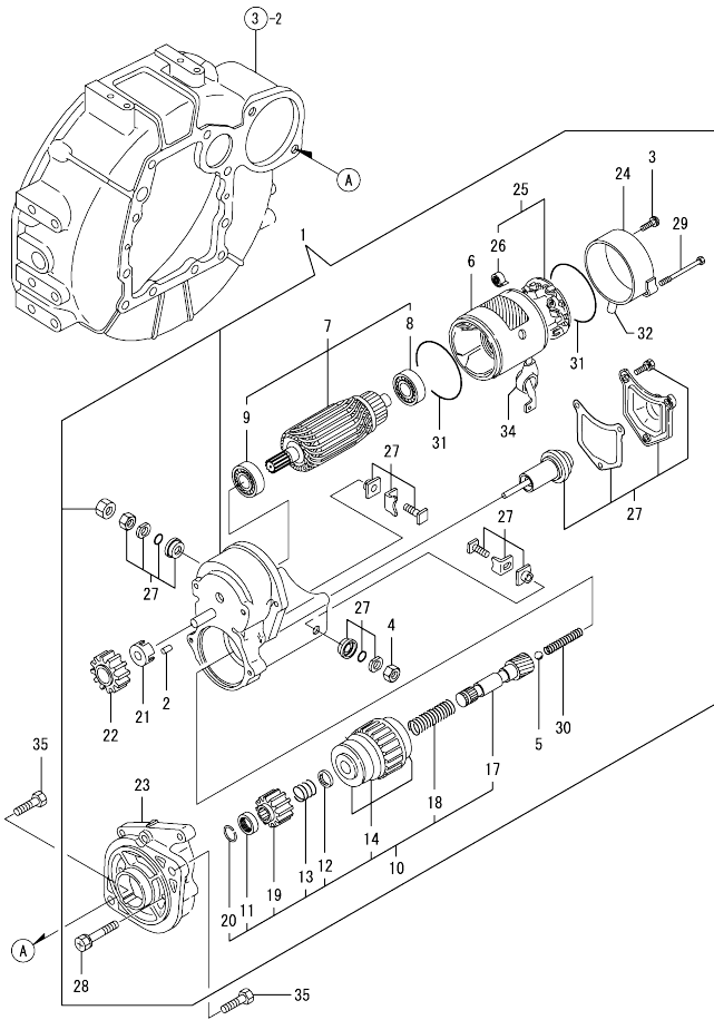
Fig.15. STARTING MOTOR
