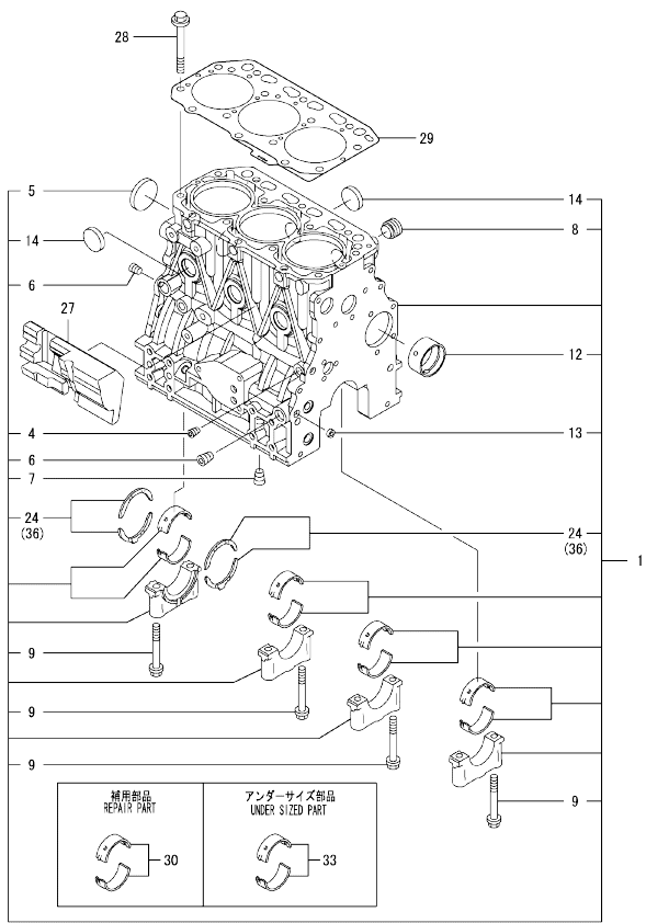
0CW10-M48100 3TNV88-GGEHC Fig.1. CYLINDER BLOCK
