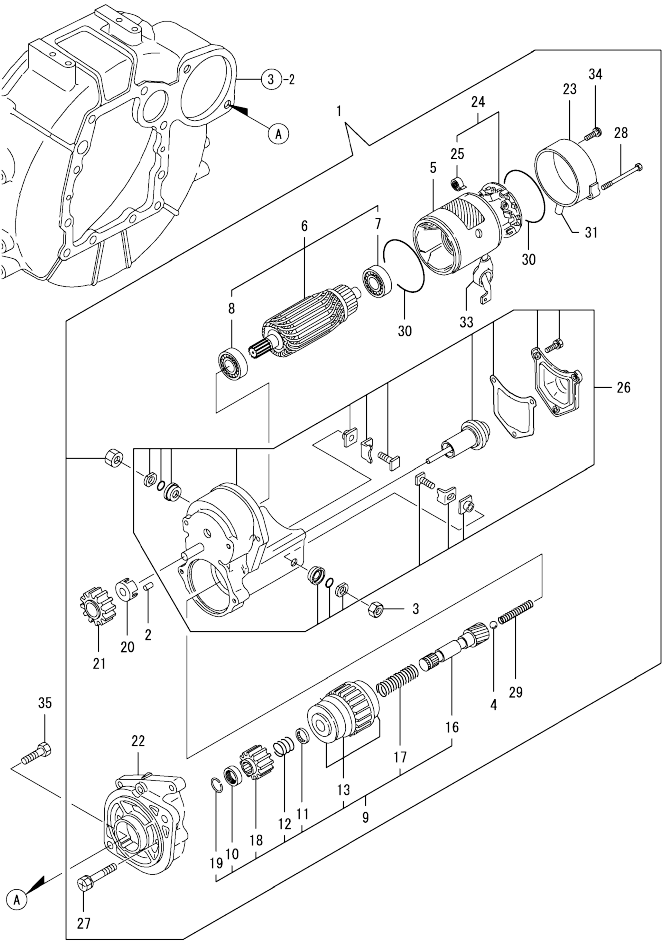
0CW10-M48100 3TNV88-GGEHC Fig.15. STARTING MOTOR
