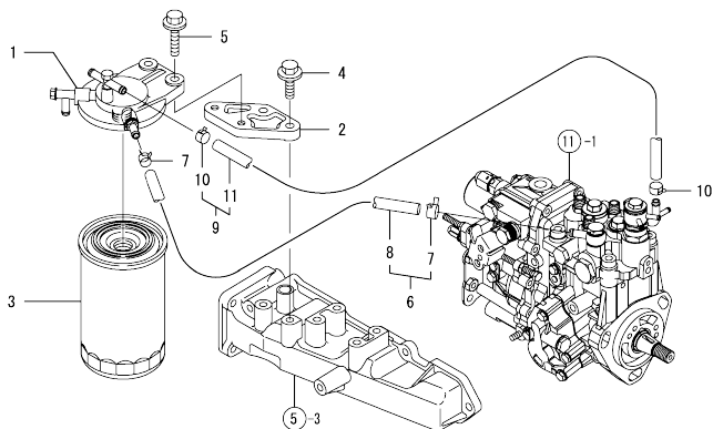
Fig.14. FUEL LINE
