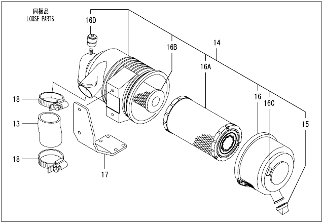
Fig.5. SUCTION MANIFOLD & AIR CLEANER
