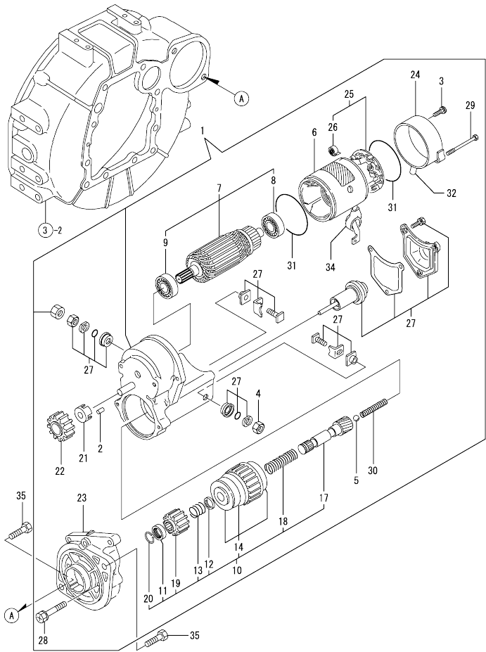
Fig.15. STARTER MOTOR
