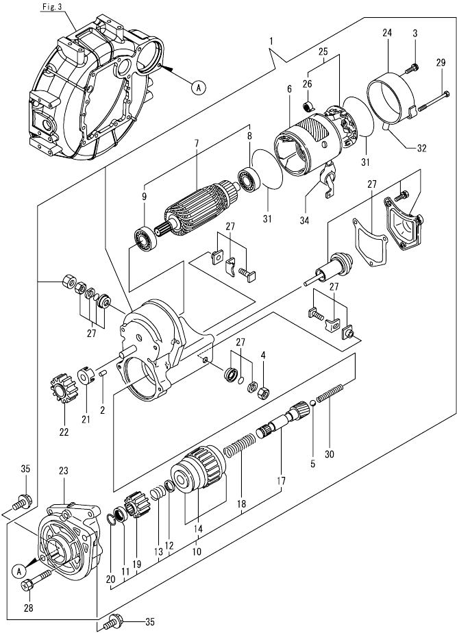
Fig.15. STARTER MOTOR
