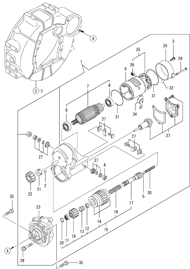
Fig.15. STARTING MOTOR
