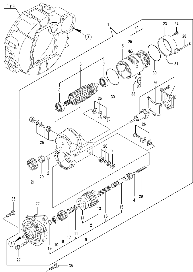
0CW10-M66800 3TNV88-KIRD Fig.15. STARTING MOTOR
