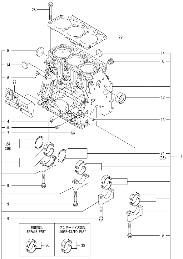
0CW10-M66800 3TNV88-KIRD Fig.1. CYLINDER BLOCK
