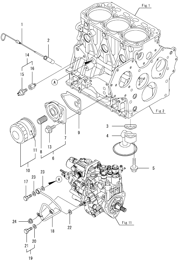
0CW10-M66800 3TNV88-KIRD Fig.9. LUB. OIL SYSTEM
