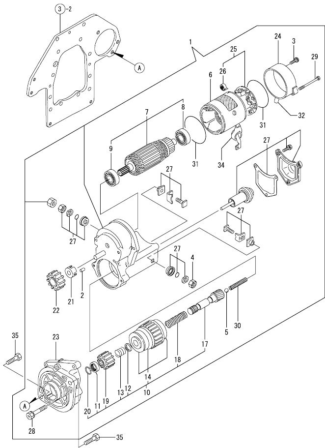
Fig.15. STARTING MOTOR
