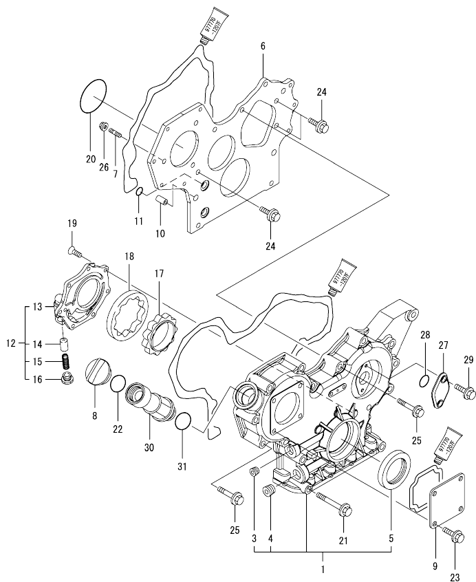
Fig.2. GEAR HOUSING
