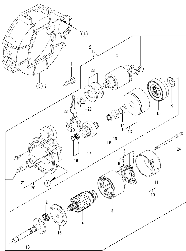
Fig.15. STARTING MOTOR
