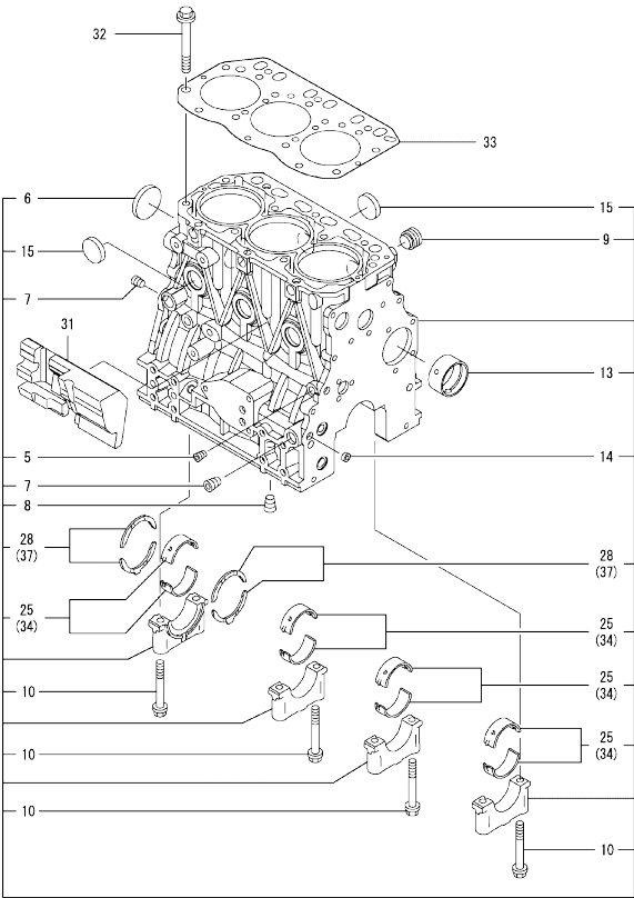
Fig.1. CYLINDER BLOCK
