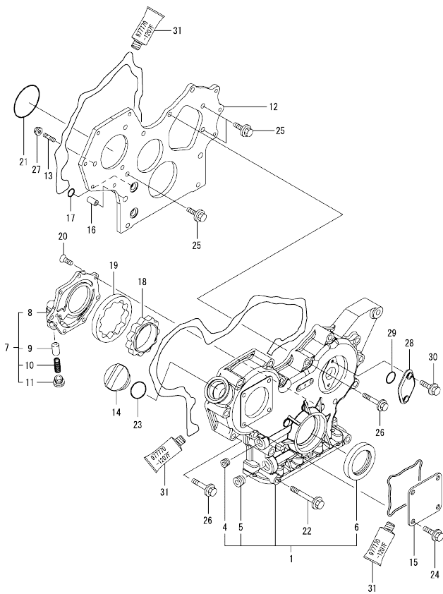
Fig.2. GEAR HOUSING
