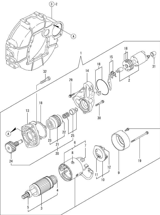
Fig.15. STARTING MOTOR
