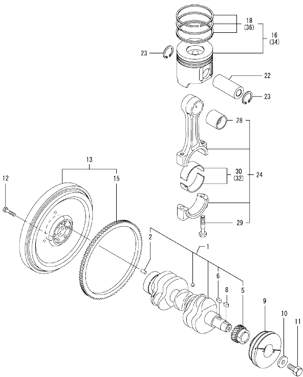
Fig.8. CRANKSHAFT & PISTON
