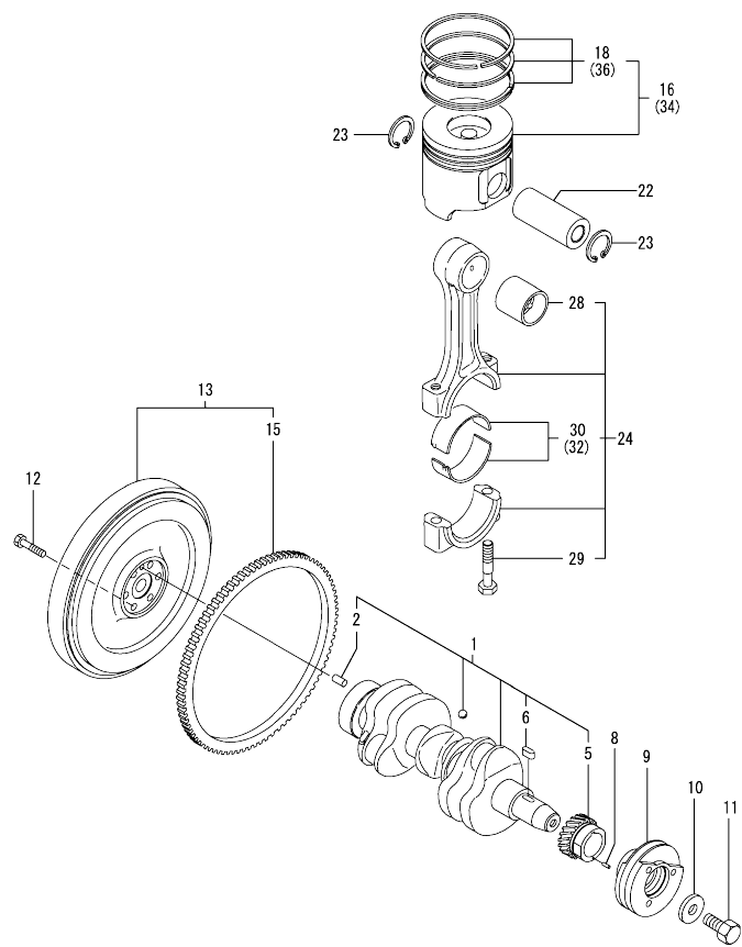
Fig.8. CRANKSHAFT & PISTON
