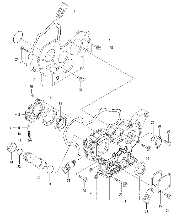
Fig.2. GEAR HOUSING
