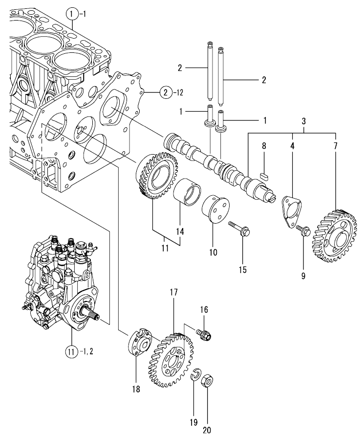
Fig.7. CAMSHAFT & DRIVING GEAR
