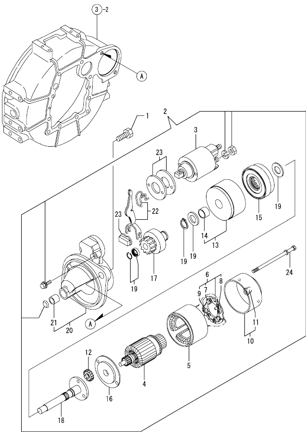
Fig.15. STARTING MOTOR
