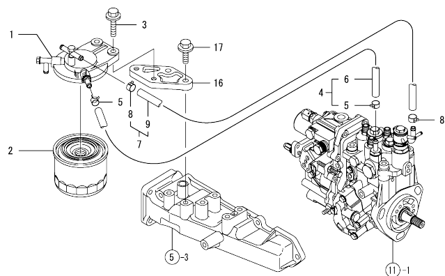
Fig.14. FUEL LINE
