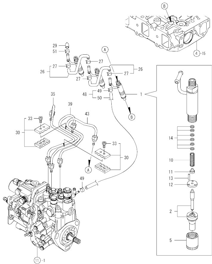
0CW10-M08600 ENGINE 3TNV88-XFU Fig.13. FUEL INJECTION VALVE
