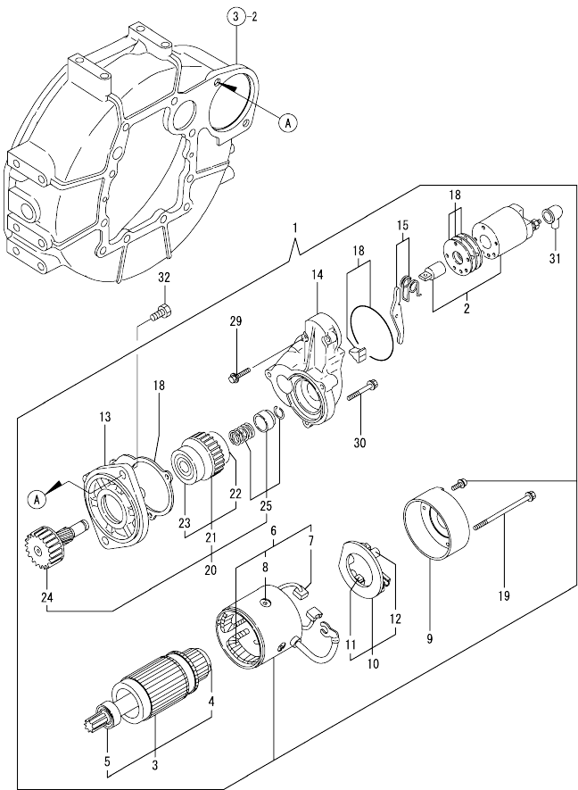
Fig.15. STARTING MOTOR
