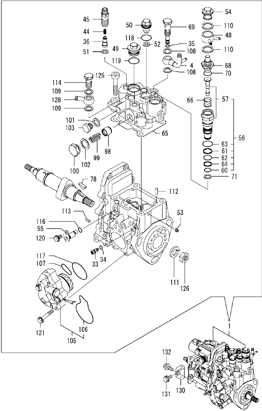
0CW10-M08600 ENGINE 3TNV88-XFU Fig.11. FUEL INJECTION PUMP
