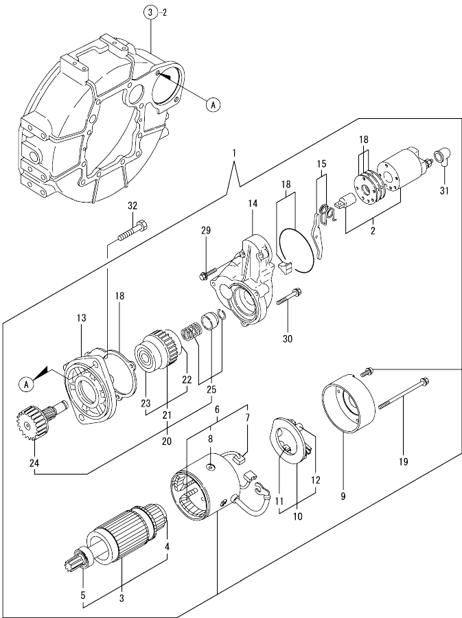
Fig.15. STARTING MOTOR
