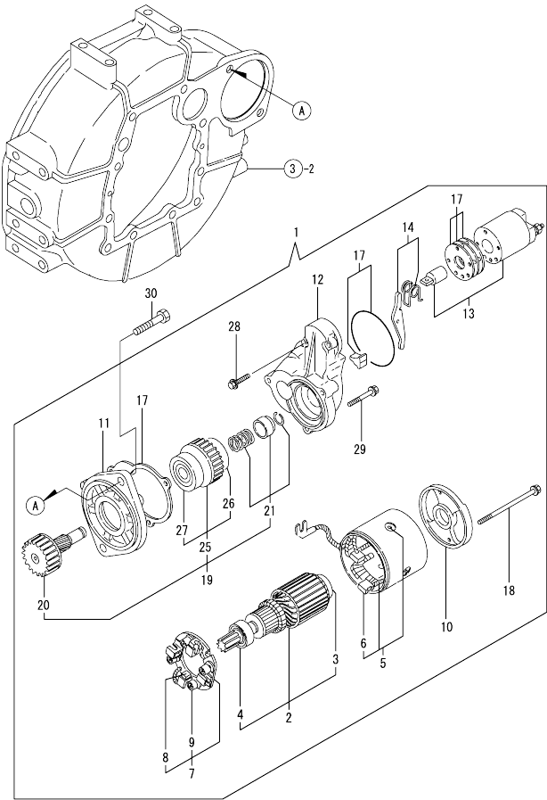
Fig.14. STARTING MOTOR
