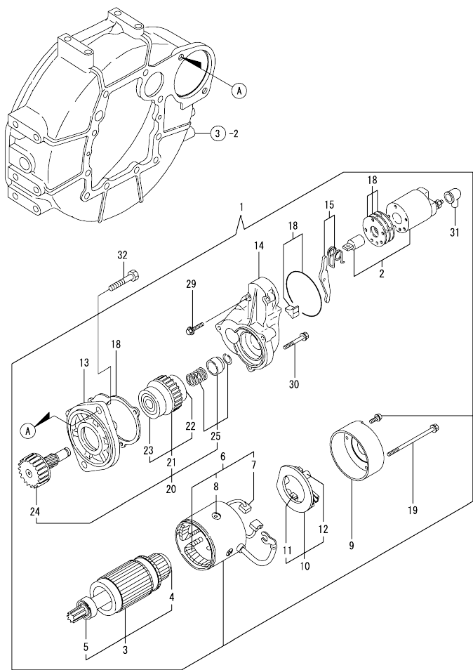
Fig.14. STARTING MOTOR
