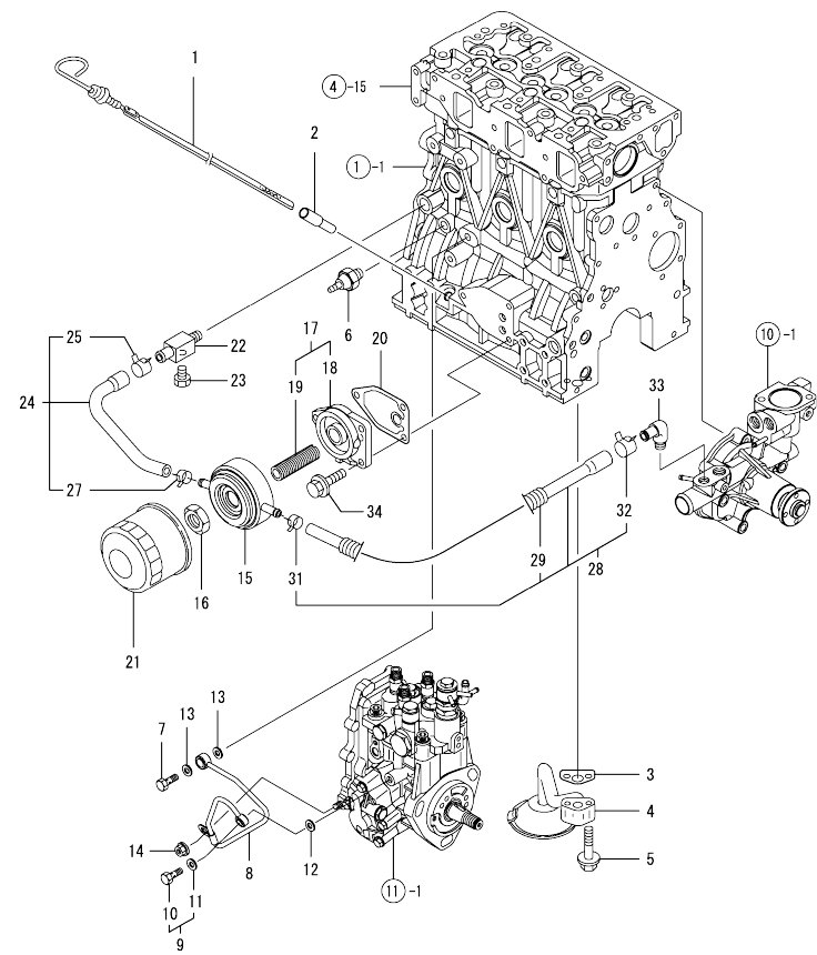
Fig.9. LUB.OIL SYSTEM
