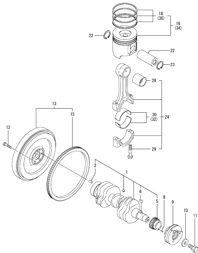
Fig.8. CRANKSHAFT & PISTON
