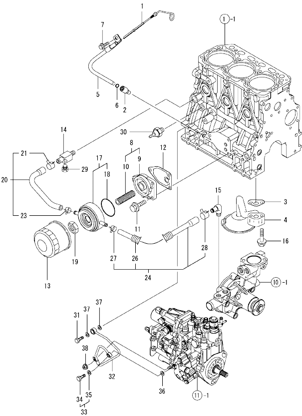
Fig.9. LUB.OIL SYSTEM
