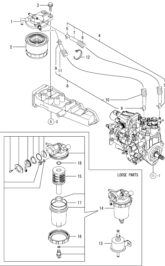
Fig.14. FUEL LINE
