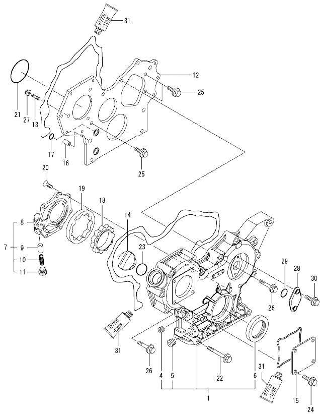
Fig.2. GEAR HOUSING
