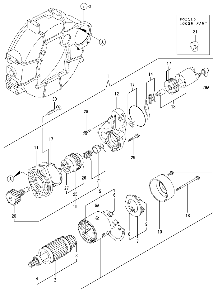
Fig.15. STARTING MOTOR
