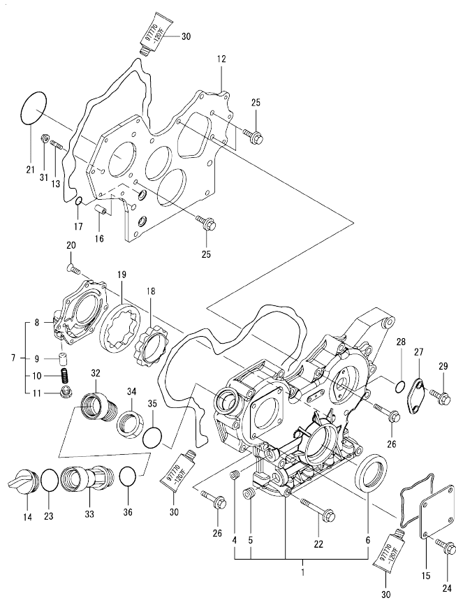
Fig.2. GEAR HOUSING
