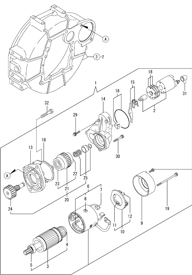
Fig.15. STARTING MOTOR
