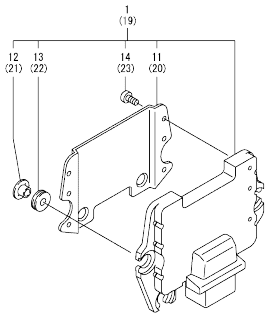
Fig.16. ELECTRONIC CONTROL UNIT(ECU)
