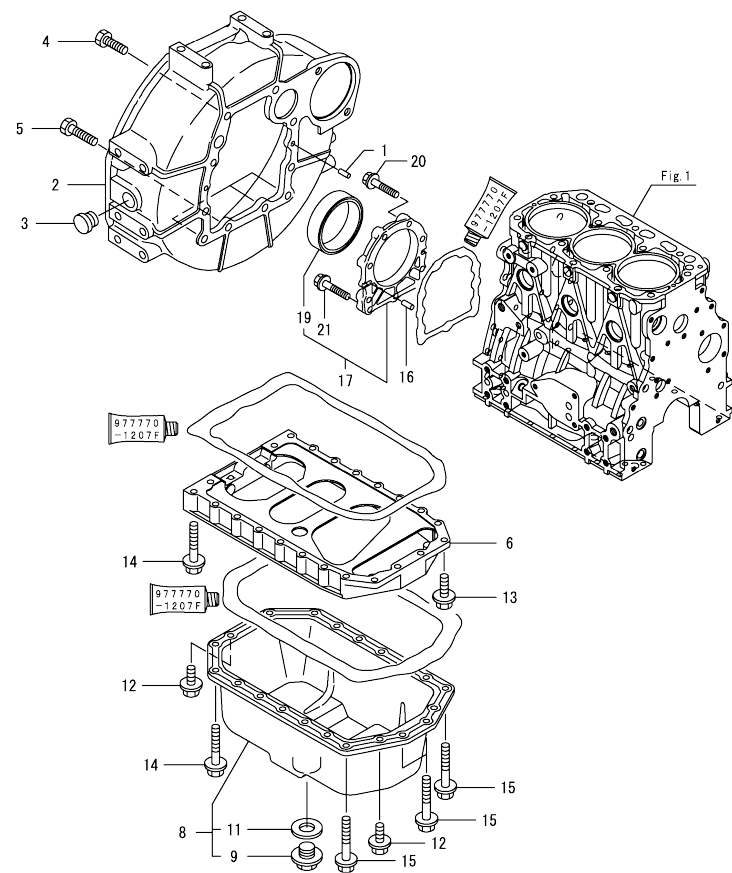
Fig.3. FLYWHEEL HOUSING & OIL SUMP
