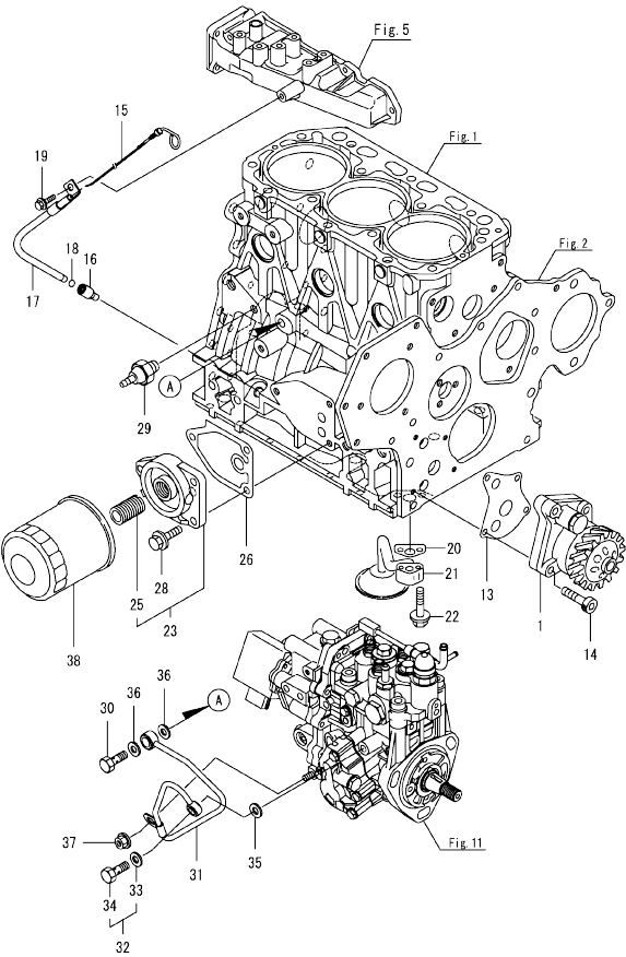
Fig.9. LUB. OIL SYSTEM
